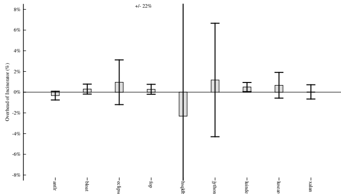
Fig. 5: Overhead of Incinerator as compared to J3 on the DaCapo 2006 benchmark applications on a low-end computer. hsqlldb has a standard deviation of 22 percentage points, truncated here for clarity.
